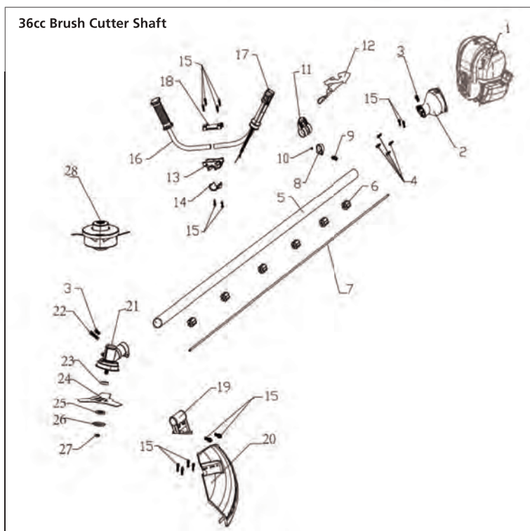
36cc Brush Cutter Shaft
